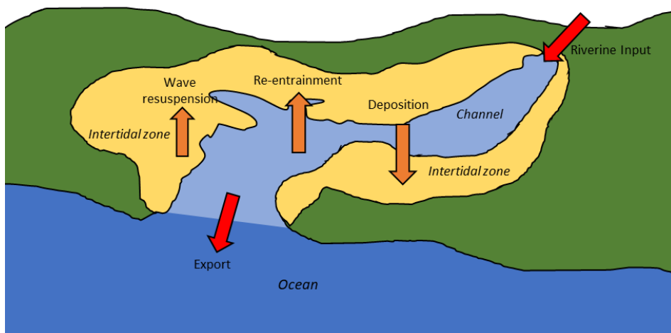
Figure 2-2: Conceptual diagram of an estuary showing the terms in the sediment mass balance model. Sediment is supplied via riverine input and exported to the sea through the mouth. A fraction deposits within the estuary. Resuspension by waves occurs on intertidal areas, and re-entrainment by currents occurs in tidal channels.
