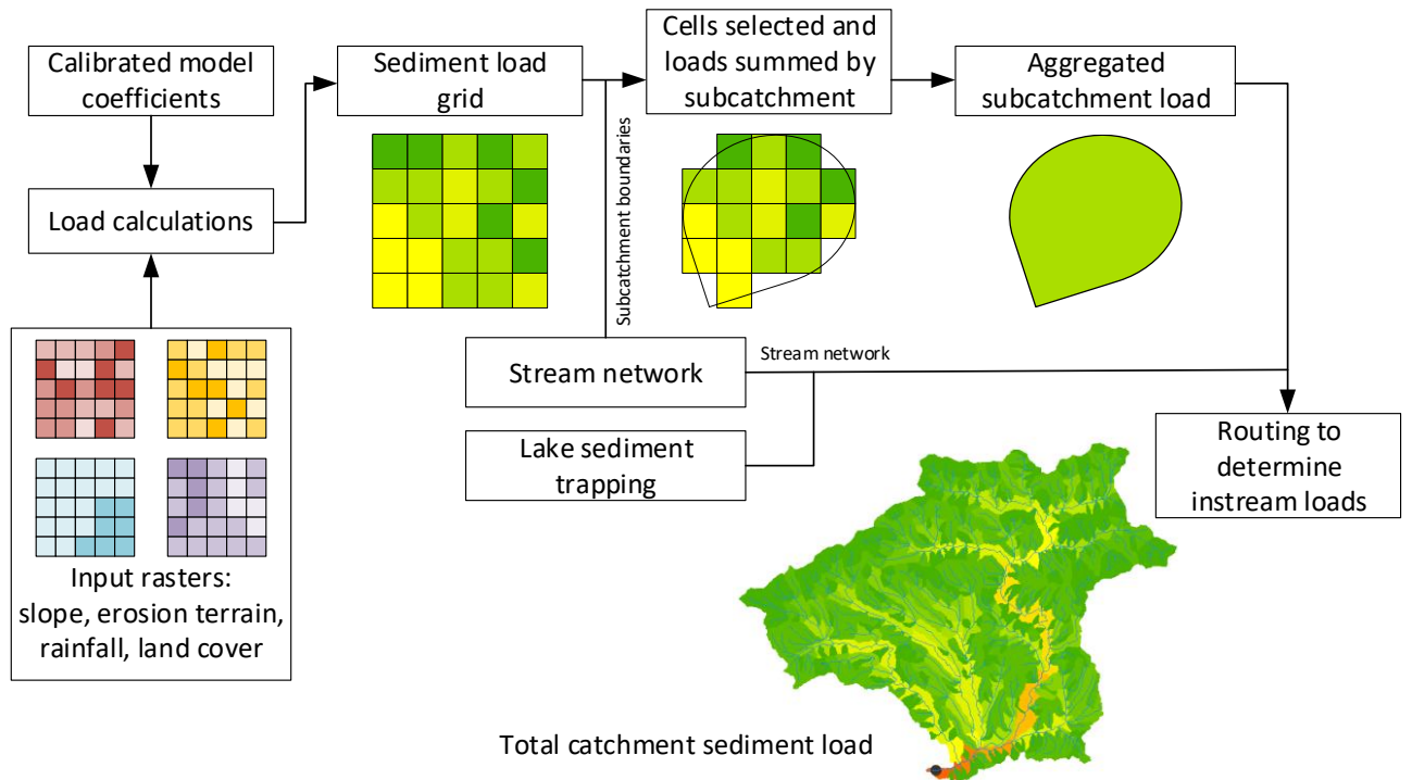
Figure 2-1: Modelling steps for the national sediment load model.
