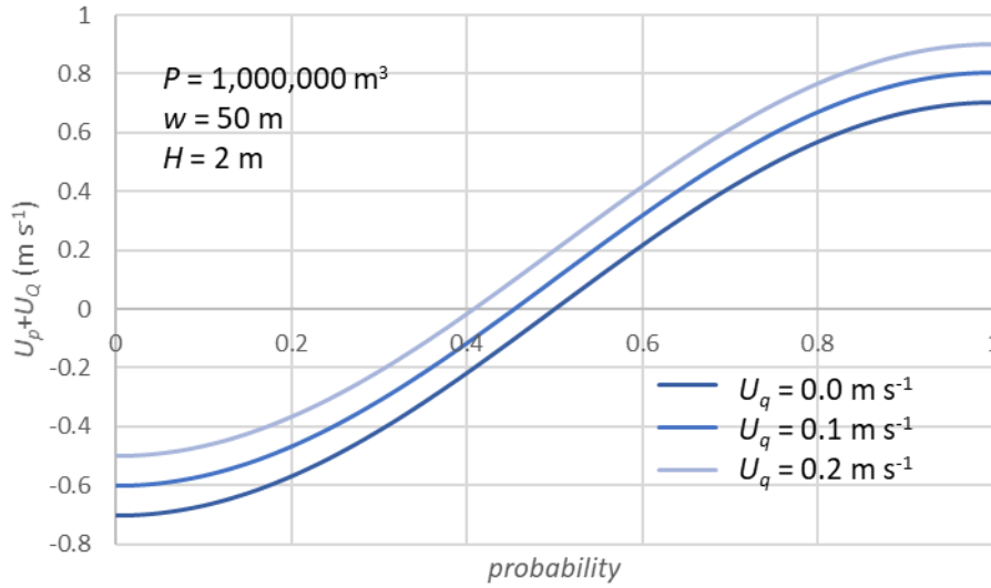
Figure A-3: Example of the probability distribution of velocities through an estuary mouth with different freshwater discharge. The example shows an estuary with tidal prism 1,000,000 m 3 , estuary mouth width 50 m depth 2 m. Tidal velocities are added to freshwater velocities of 0, 0.1, and 0.2 m/s, which would represent daily freshwater discharges of 0, 10, and 20 m 3 /s.
