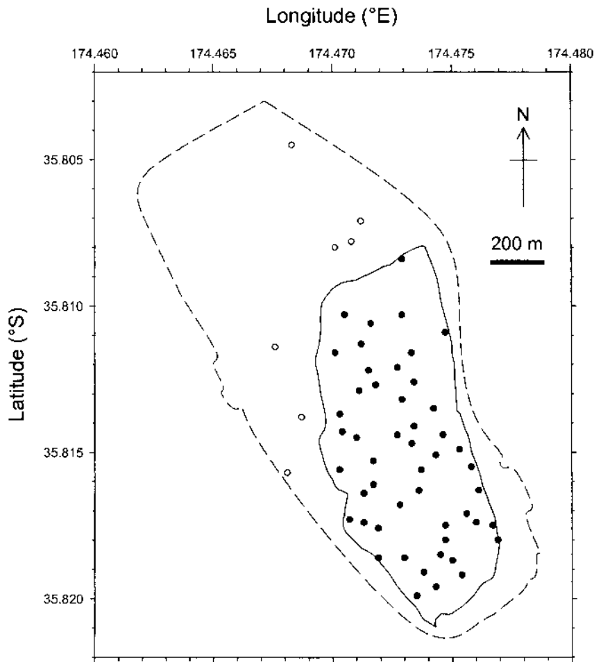
Figure 2: Design of the March 2005 cockle survey on Snake Bank, Whangarei Harbour. Filled circles indicate site positions ( n = 50 ) in the high density stratum (solid line) and open circles denote sites ( n = 7 ) in the low density stratum (dashed line). The boundary of the high density stratum was estimated by walking the perimeter of the bank at a reasonably low tide (0.5 m chart datum) and periodically recording positions using GPS. The low density stratum boundary was determined by Morrison & Cryer (1999), and is likely to be inaccurate because it has not been measured recently. Latitude and longitude are in decimal degrees.
