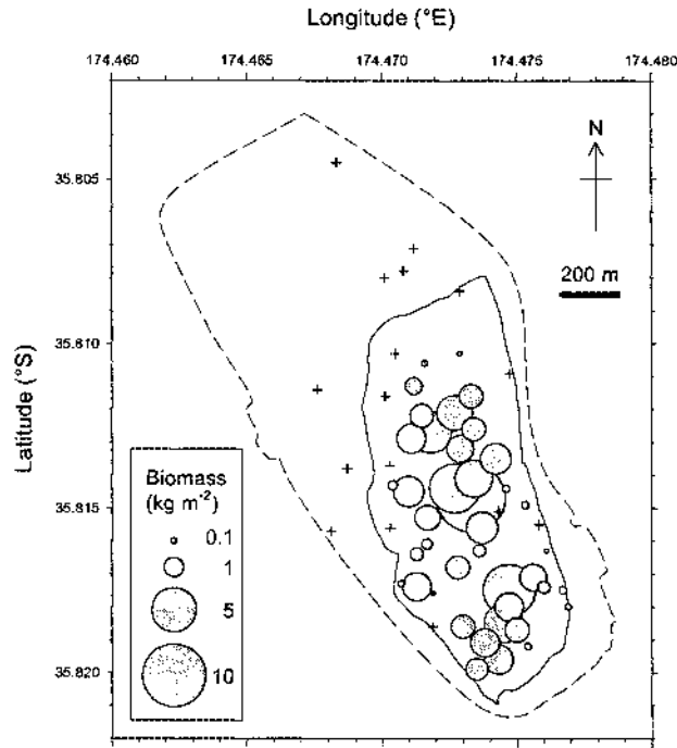
Figure 4: Distribution of cockle biomass on Snake Bank, Whangarei Harbour, 2005. Filled circles indicate sites sampled in the high density stratum (solid line) where cockles were present; circle area is proportional to the estimated biomass ( \text{kg m}^{-2} ) of cockles at each site. Crosses denote those sites sampled with zero cockles. Zero cockles were found in the seven sites sampled in the low density stratum (dashed line). Latitude and longitude are in decimal degrees.
