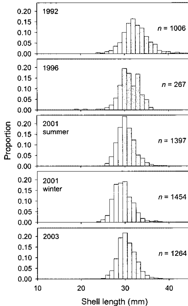
Figure 7: Estimated length frequency distribution of cockles in the commercial harvest from Snake Bank in 1992 (Cryer 1997), 1996 (Cryer 1997), 2001 (Cryer and Parkinson 2001) and 2003 (Cryer et al. 2004). The shaded part of each histogram contains cockles 30 mm SL and larger (the nominal size at recruitment to the fishery).
