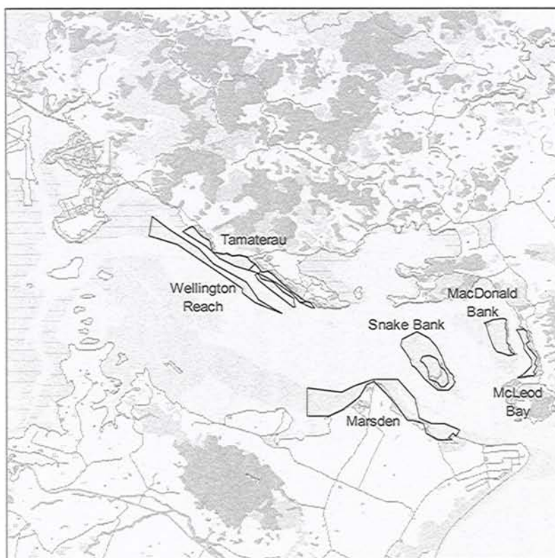
Figure 1: Beaches and banks within Whangarei Harbour that support appreciable numbers of cockles (as at July 2002, Cryer et al. (2002b)). Sampling strata are delineated by solid lines. The boundary of Snake Bank has subsequently moved (see Figure 5).
