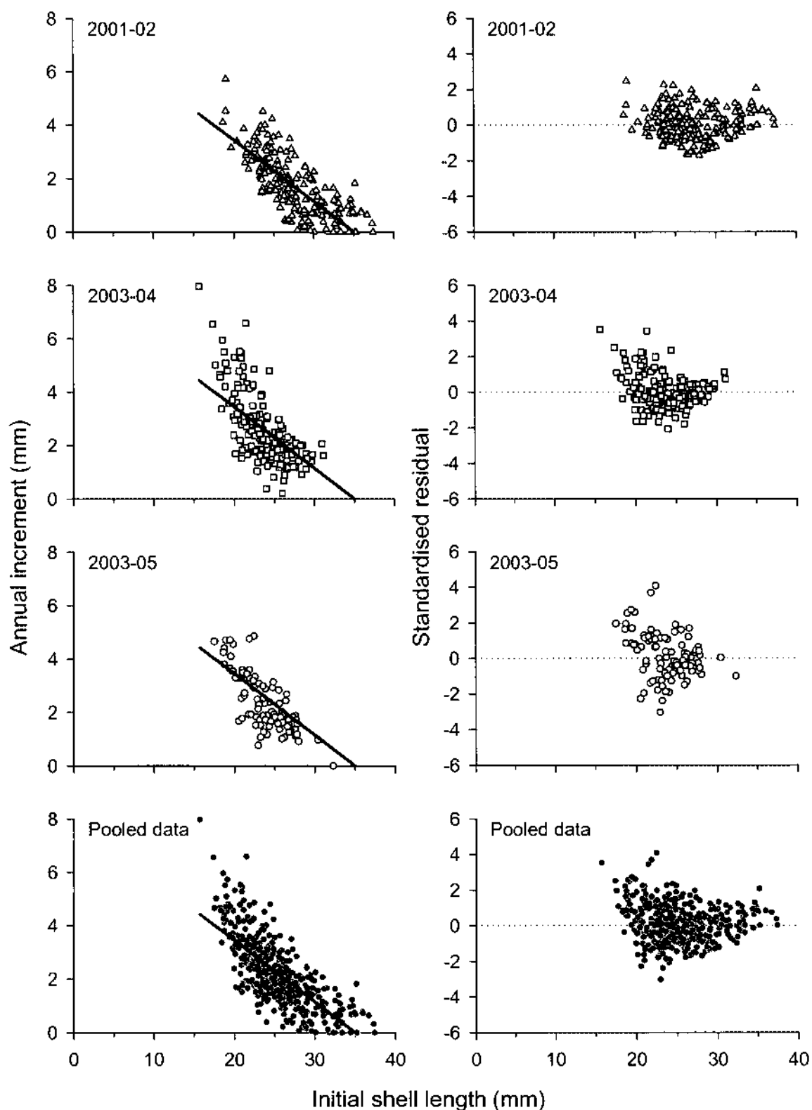
Figure 8: Incremental growth data and standardised residuals from the fitted GROTAG model (Francis 1988) for notch tagged cockles on Snake Bank, Whangerei Harbour, 2001–2005. The solid black line represents the model fitted to the data pooled from the 2001–02 ( n = 191 ), 2003–04 ( n = 178 ) and 2003–05 ( n = 96 ) tag-recapture experiments. The observed increments have been scaled to reflect expected annual growth.
