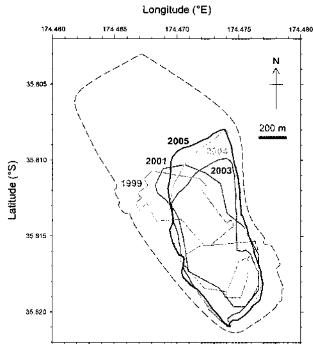
Figure 5: Location of the high density sampling strata on Snake Bank between 1999 and 2005 showing movement to the east, at least for the northern part of the stratum. The 1999 stratification was a modified version of the 1998 stratification which, in turn, was based on the average distribution of cockles 1985–96. Dashed line indicates the low density stratum boundary. Latitude and longitude are in decimal degrees.
