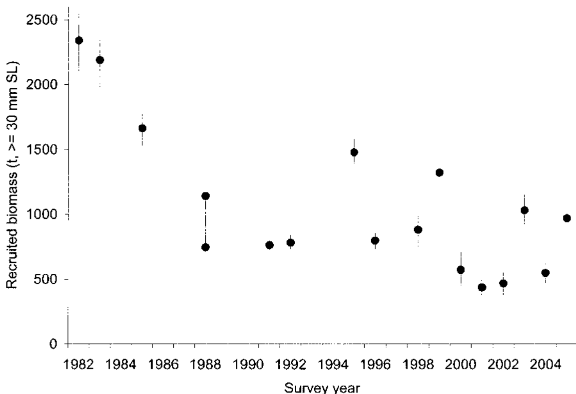
Figure 3: Estimated recruited biomass of cockles (30 mm or more SL, \pm one standard error) on Snake Bank from surveys between 1982 and 2005. The 1988 grid survey was abandoned part-way through and its analysis is complicated; two alternative analytical approaches are plotted as dots. The 2001 result comes from the second of two surveys, the first (in April) having produced unacceptably imprecise results.
