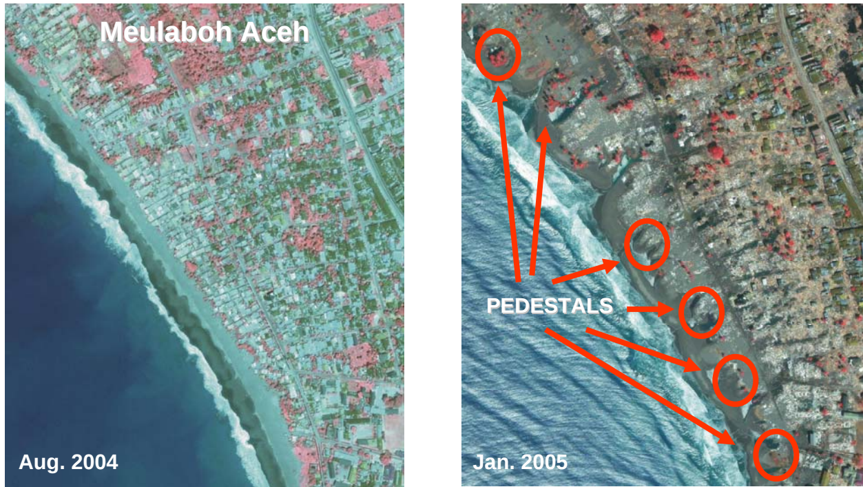
Figure 24: Pedestal formation in Aceh Province, December 26 th 2004 (Images from http://www.crisp.nus.edu.sg/tsunami/tsunami.html , they were acquired and processed by CRISP, National University of Singapore. IKONOS image © CRISP 2004).
