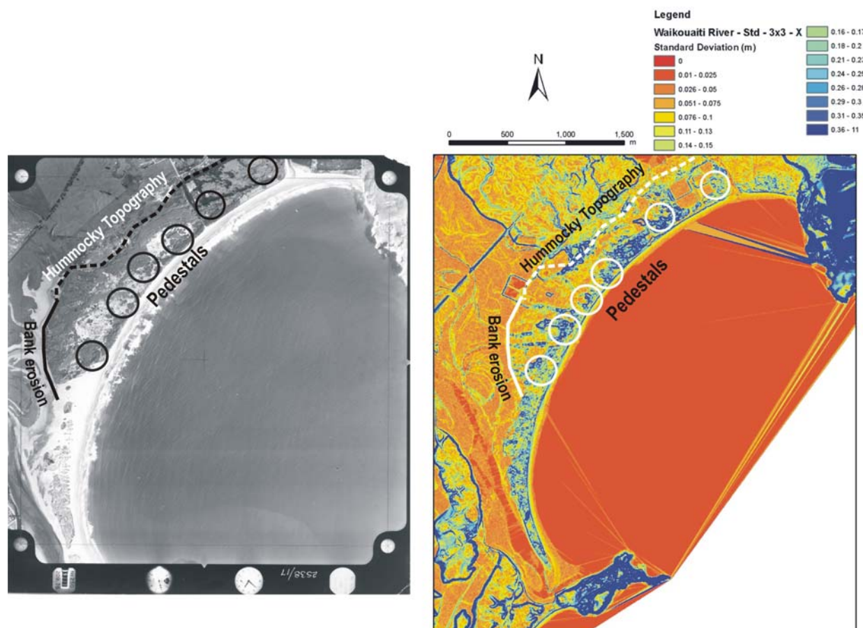
Figure 47: Annotated images of the Waikouiti coastline: A 1958 aerial photograph on the left and 2005 LIDAR image ('X-cross' filtering method) on the right (Photo courtesy of Otago Regional Council).
