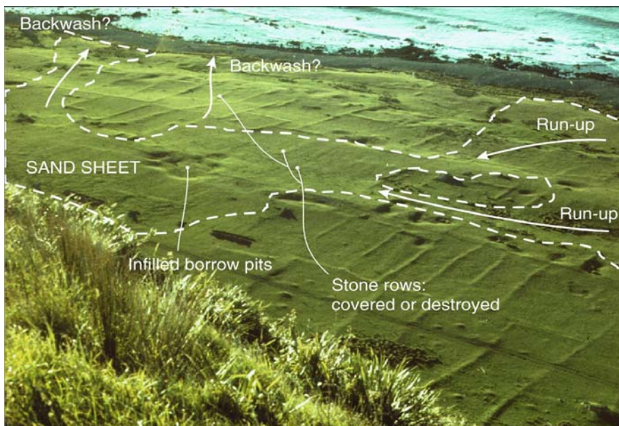
Figure 27: Wairarapa coast: landward sand sheet in limited accumulation space, 15 th century (Photo G. Billing, © B. McFadgen).
