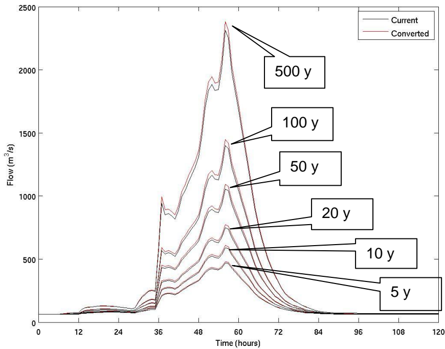
Figure 66 Simulated Taupo-Karapiro inflow hydrographs (TopNet) for the 6 synthetic rainfall events under current (black) and converted (red) land use scenarios, 1958 events
