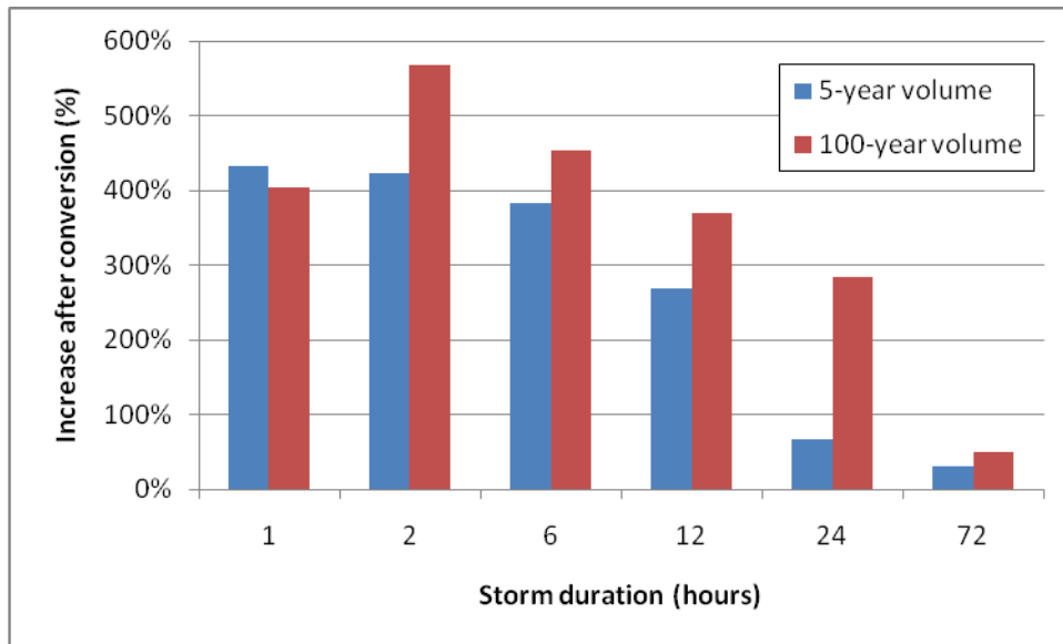
Figure 55 Pokaiwhenua at SH1: Increase in runoff volume after conversion on HEC-HMS
