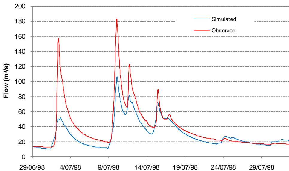
Figure 33 Simulated and observed flows for Mangakino at Dillon Rd calibration (July 1998 flood)
