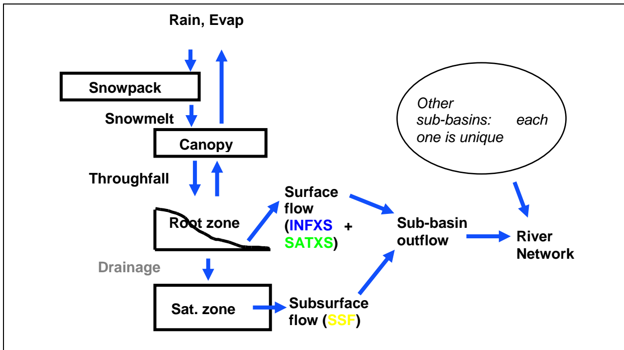
Figure 8 Overview of TopNet model structure showing the snowpack, canopy, root zone, saturated zone and river network components of the model. Arrows indicate flows of water from one model component to another.
