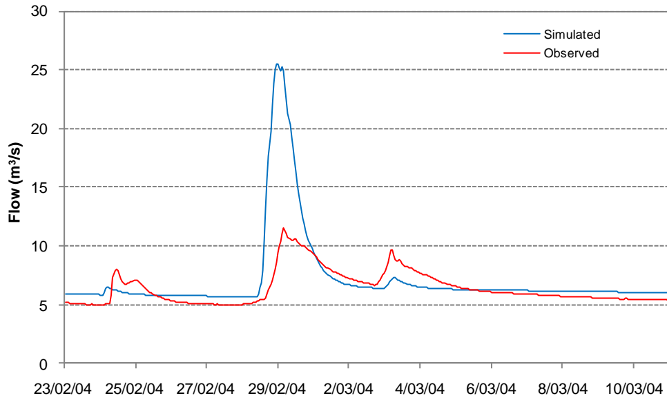
Figure 38 Observed and simulated flow at Pokaiwhenua at Puketuria calibration for the February 2004 flood
