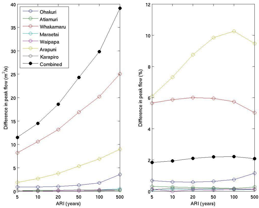
Figure 59 Peak flow differences in m^3/s (left) and percent (right) for the converted scenarios compared to current land use hydrographs (TopNet simulations, 1998 rainfall pattern). Results are displayed for different return intervals and the dam catchments as well as the outlet. “Combined” refers to the total Taupo-Karapiro inflows.
