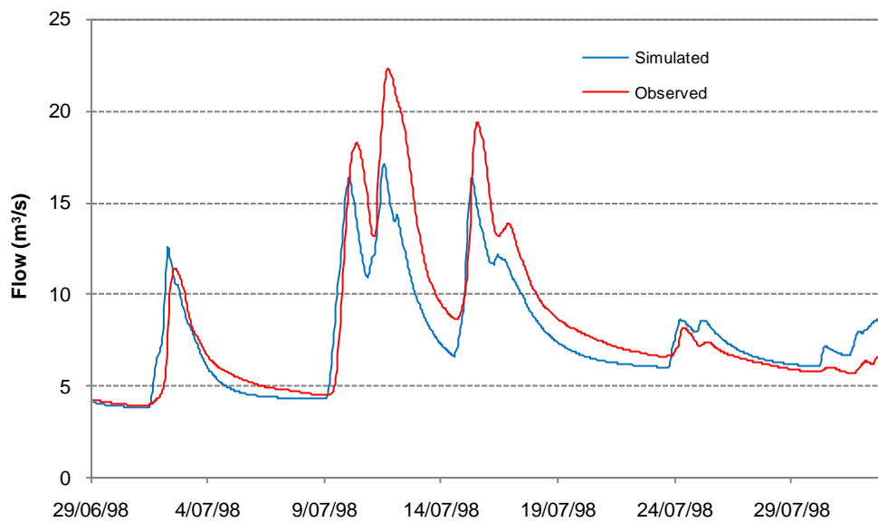
Figure 25 Observed and simulated flows for Waitotapu at Reporoa calibration (July 1998 flood)
