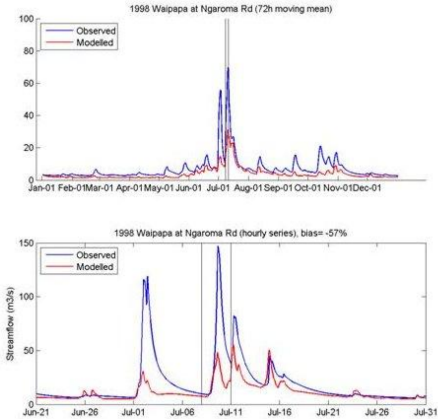
Figure 20 TopNet validation plot for 1998 flood, Waipapa at Ngaroma Road. Top panel shows observed and modelled 72-h moving mean flows in m^3 s^{-1} ; Bottom panel shows observed and modelled hourly flows in m^3 s^{-1}
