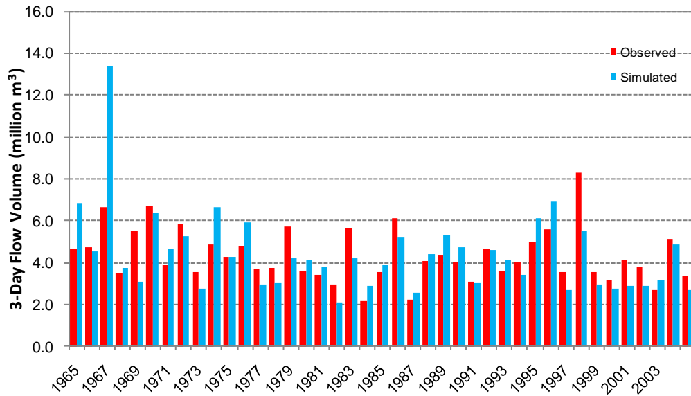
Figure 28 Observed and simulated 3-day flow volume annual maxima for Tahunaatara at Ohakuri calibration
