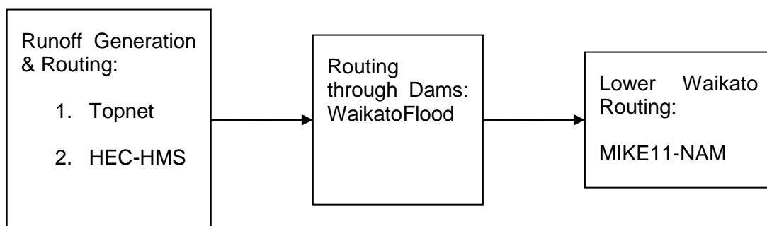
Figure 6 Schematic of the models used in this study
