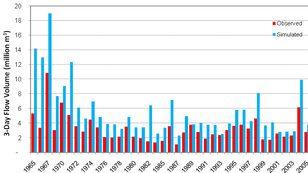
Figure 12 Observed and simulated 3-day flow volume annual maxima for Waio tapu at Reporoa calibration
