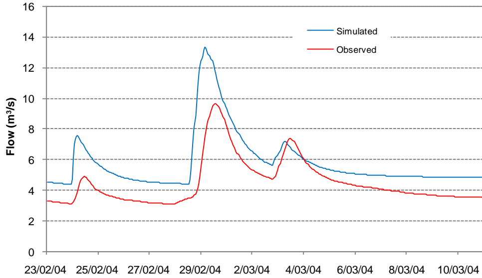
Figure 26 Observed and simulated flows for Waiotapu at Reporoa calibration (February 2004 flood)
