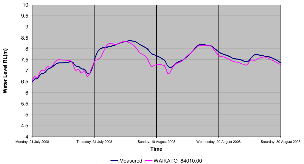
Figure 50 Measured and modelled flood levels at Hamilton and Rangiriri, for August 2008 calibration event
