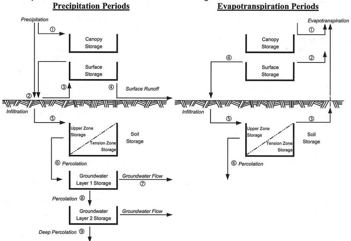
Figure 10 Operation of the SMA model (sourced from Bennett and Peters, 2000)
