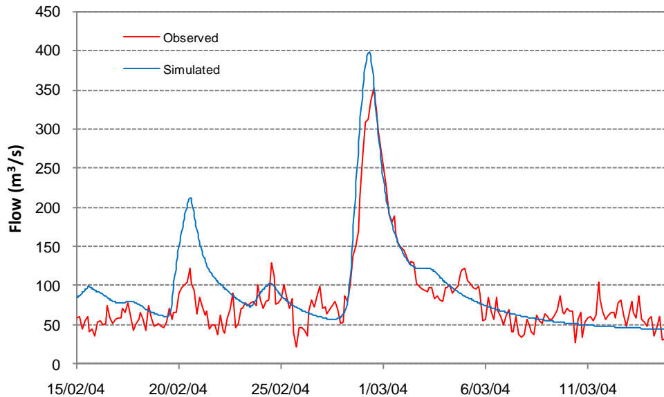
Figure 44 Simulated and observed inflow to the catchment between Lakes Whakamaru and Karapiro for the February 2004 flood event (24-hour moving mean)
