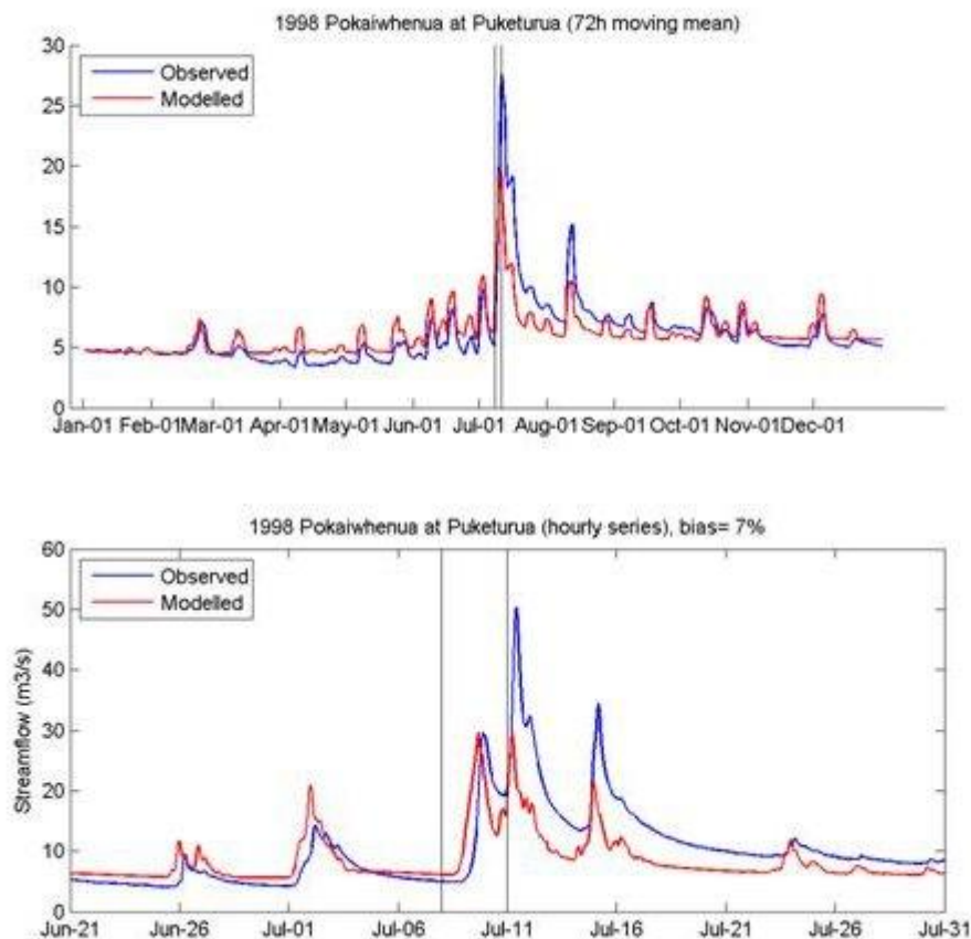
Figure 21 TopNet validation plot for 1998 flood, Pokaiwhenua at Puketurua. Top panel shows observed and modelled 72-h moving mean flows in \text{m}^3\text{s}^{-1} ; Bottom panel shows observed and modelled hourly flows in \text{m}^3\text{s}^{-1}
