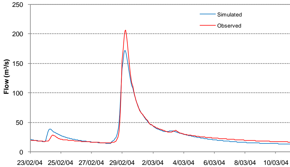
Figure 34 Simulated and observed flows for Mangakino at Dillon Rd calibration (February 2004 flood)
