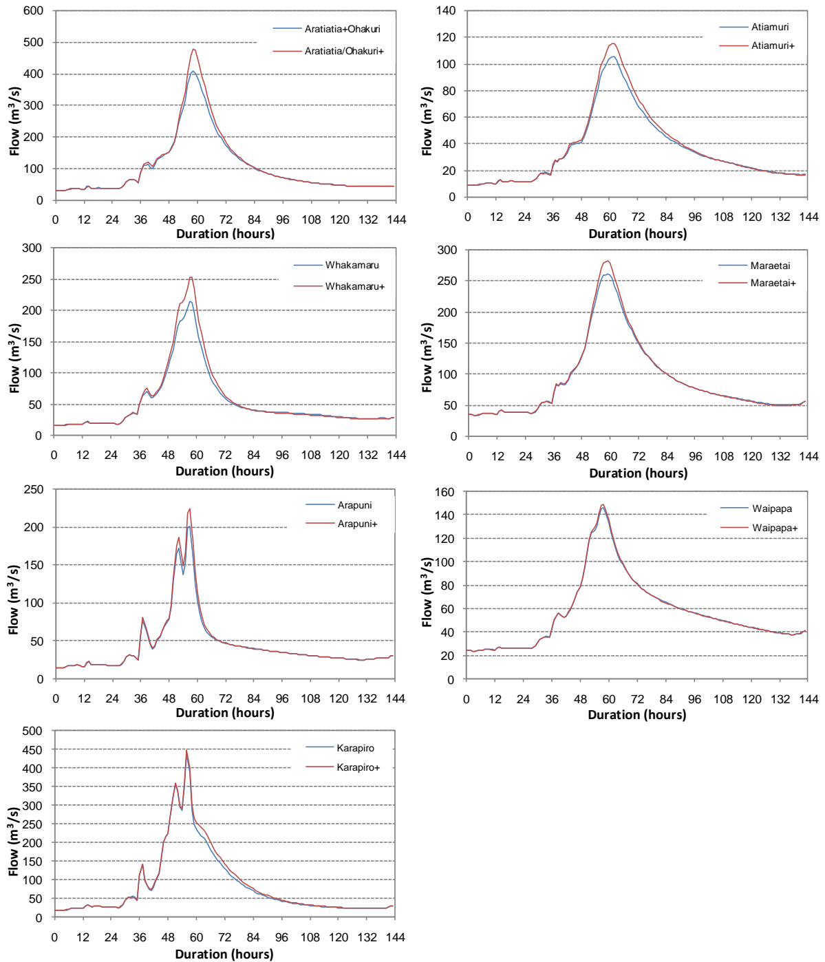
Figure 62 Effect of land use change (indicated by + symbol) on dam catchment inflows for 100-year test event for 1958 on 7 dam catchments, using HEC-HMS
