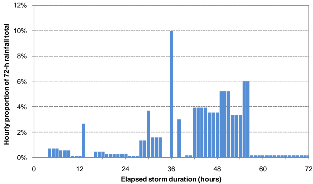
Figure 53 72-hour temporal pattern of the February 1958 storm rainfall event
