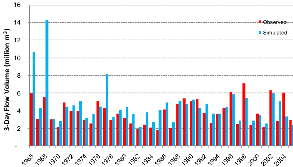
Figure 36 Observed and simulated 3-day flow volume annual maxima for Pokaiwhenua at Puketuru calibration
