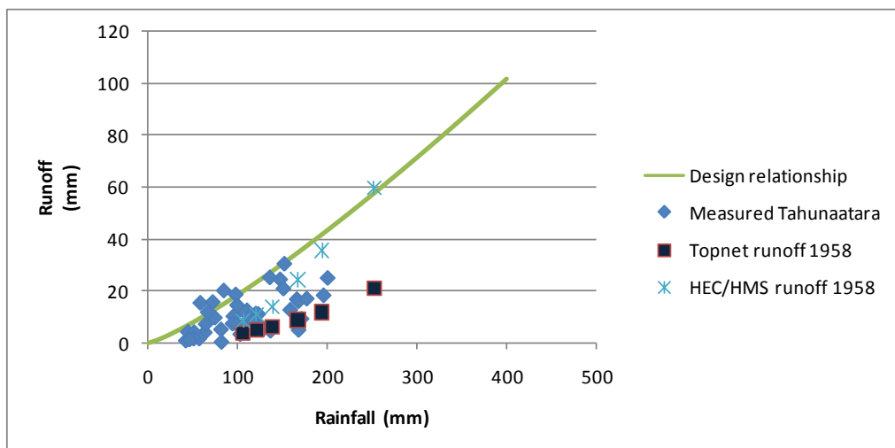
Figure 46 Measured storm runoff produced by total storm rainfalls and maximum design relationship in the Tahunaatara Stream compared to storm runoff into Atiamuri reservoir predicted by HEC-HMS and TopNet models for rainfalls of 5 to 500 year ARI with 1958 temporal pattern
