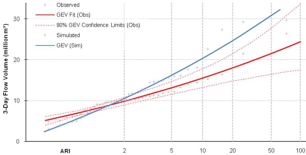
Figure 15 Distribution of observed and simulated 3-day flow volume annual maxima for Mangakino at Dillon Road calibration (using Gringorton plotting positions)
