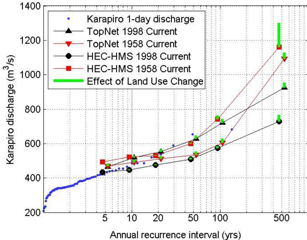
Figure 69 The data and model results as in Figure 68 but with the future land use scenarios added (green bars).
