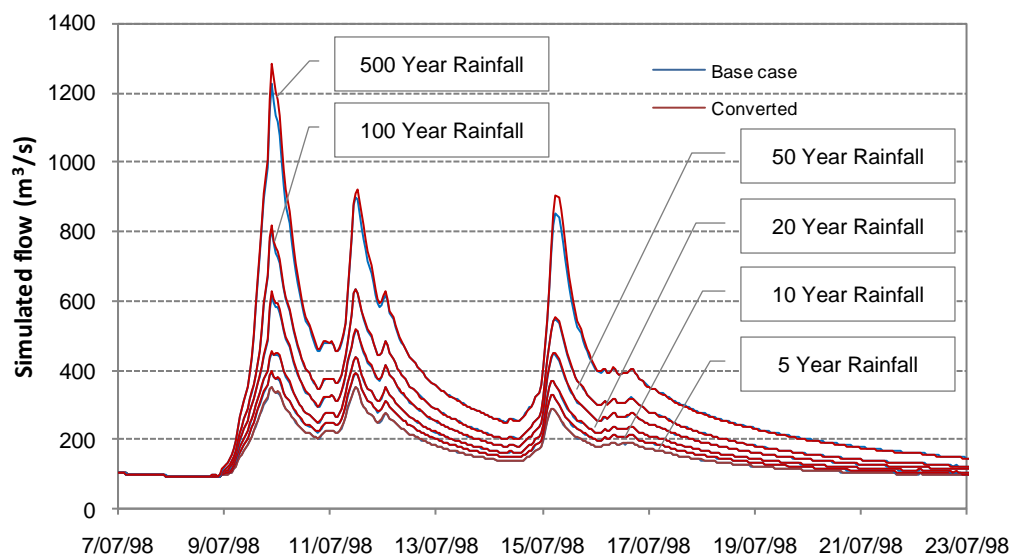
Figure 63 Simulated Taupo – Karapiro inflow hydrographs of six notional magnitude storm events under base case and converted land use scenarios, HEC-HMS, 1998 events
