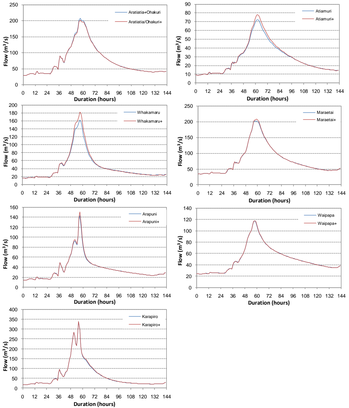
Figure 61 Effect of land use change (indicated by + symbol) on dam catchment inflows for 50-year test event for 1958 on 7 dam catchments, using HEC-HMS
