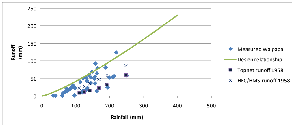
Figure 48 Measured storm runoff produced by total storm rainfalls and maximum design relationship in the Waipapa River compared to storm runoff into
