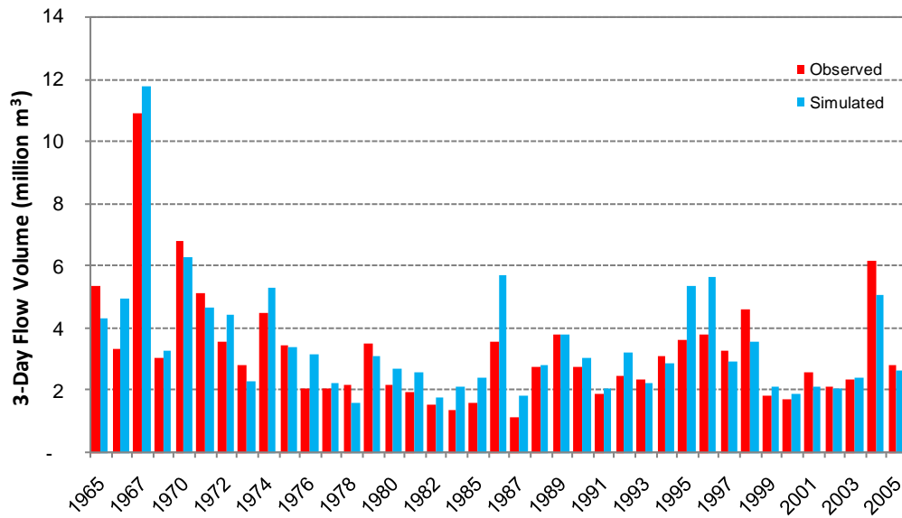
Figure 24 Observed and simulated 3-day flow volume annual maxima for Waitotapu at Reporoa calibration
