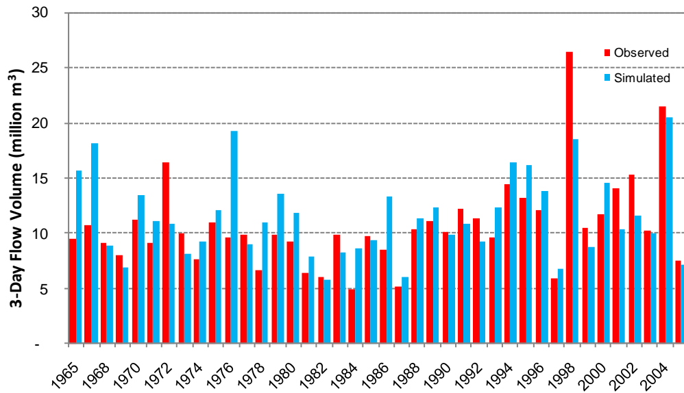
Figure 32 Observed and simulated 3-day flow volume annual maxima for Mangakino at Dillon Rd calibration
