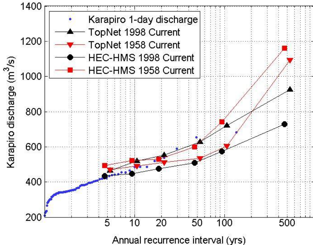
Figure 68 Recorded annual maximum 1 day discharges and associated annual recurrence intervals from Karapiro compared with simulated discharges resulting from HEC-HMS and TopNet simulated inflows for the current land use, and with temporal patterns matching both the 1998 and 1958 storms. TopNet and HEC-HMS results are horizontally offset from the exact ARI for the sake of clarity.
