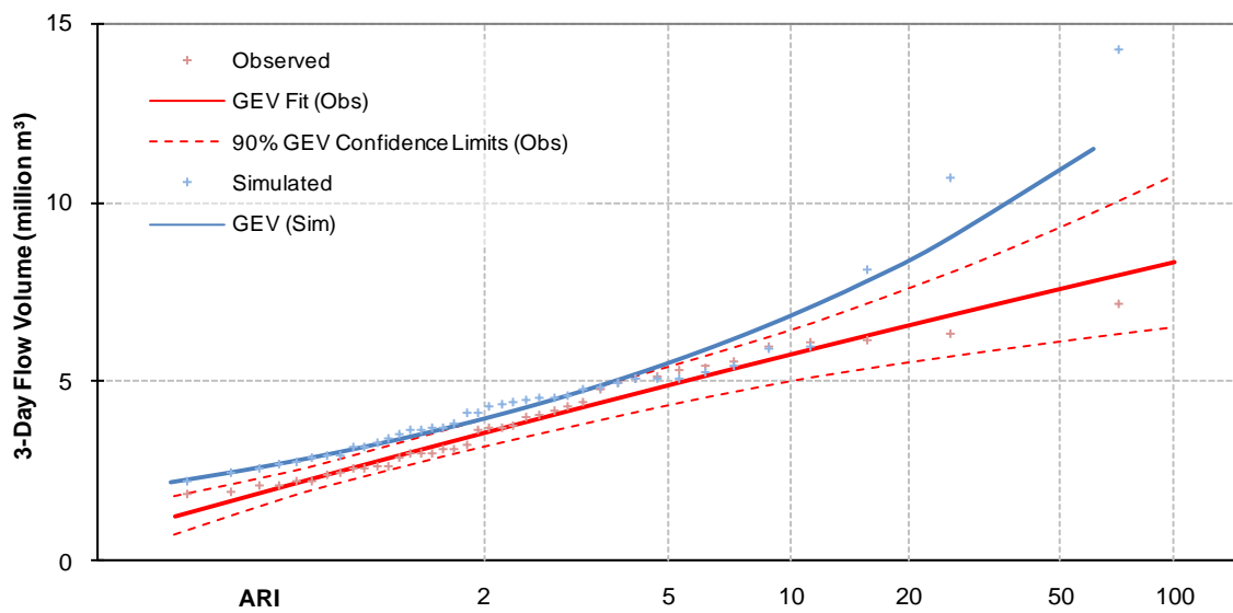
Figure 35 Distribution of observed and simulated 3-day flow volume annual maxima for Pokaiwhenua at Puketurua calibration (using Gringorton plotting positions)
