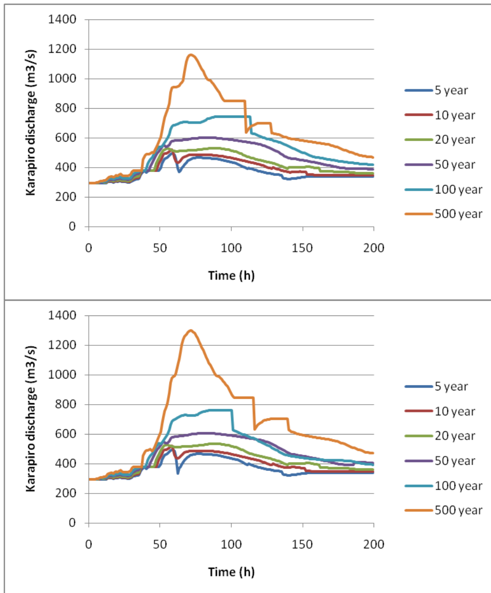
Figure 67 Hydrographs of Karapiro discharge simulated using HEC-HMS model inflow hydrographs for 5-500 year rainfalls with 1958 temporal pattern with current land use (above) and with future land use (below) scenarios
