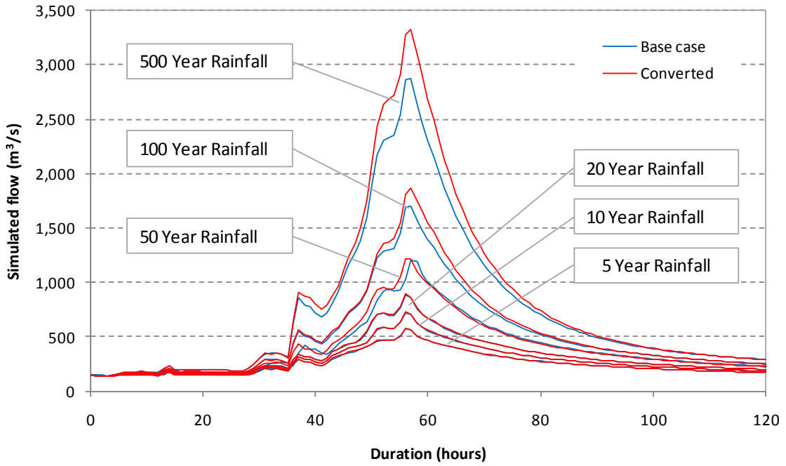
Figure 65 Simulated Taupo – Karapiro inflow hydrographs of six notional magnitude storm rainfall events under base case and converted land use scenarios, 1958 events
