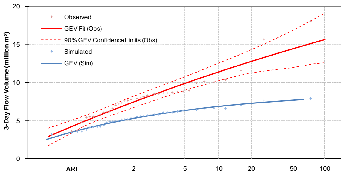
Figure 39 Distribution of observed and simulated 3-day flow volume annual maxima for Waipapa at Ngaroma Rd calibration (using Gringorton plotting positions)
