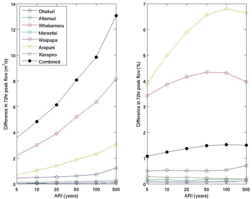
Figure 60 Peak 72-hr flow differences in m^3/s (left) and percent (right) for the converted scenarios compared to current land use hydrographs (TopNet simulations, 1998 rainfall pattern). Results are displayed for different return
