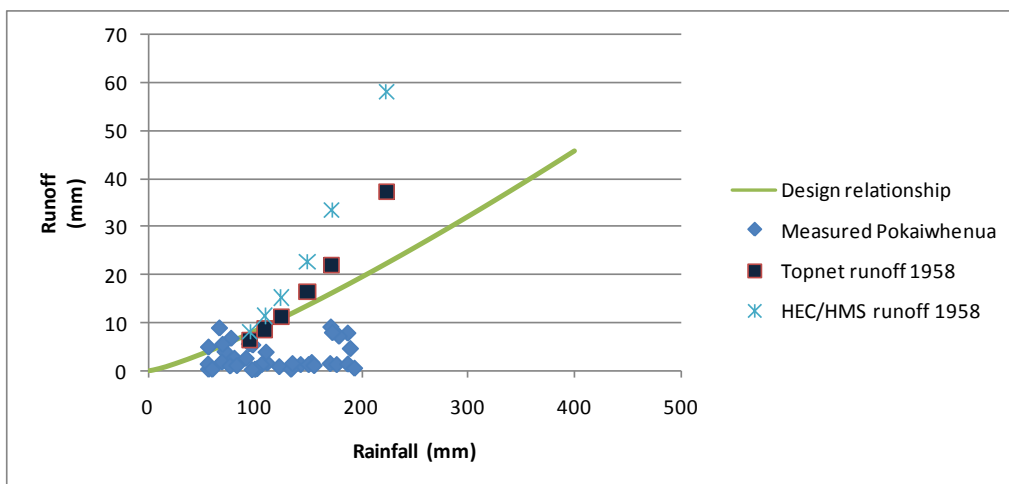
Figure 49 Measured storm runoff produced by total storm rainfalls and maximum design relationship in the Pokaiwhenua Stream compared to storm runoff into Karapiro reservoir predicted by HEC-HMS and TopNet models for rainfalls of 5 to 500 year ARI with 1958 temporal pattern
