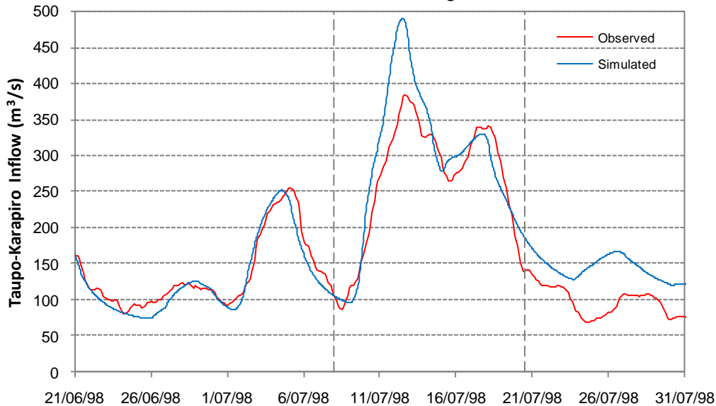
Figure 40 Observed difference between Taupo and Karapiro outflows and simulated catchment flow for the 1998 flood event (72-hour moving means)
