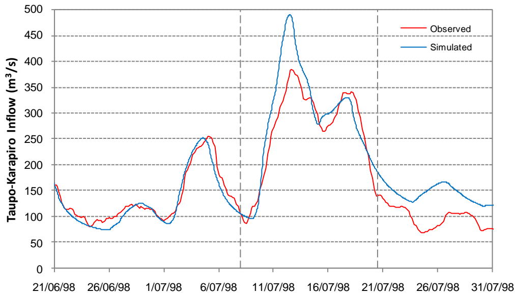
Figure 22 Observed difference between Taupo and Karapiro outflows and simulated catchment flow for the 1998 flood event (72-hour moving means)
