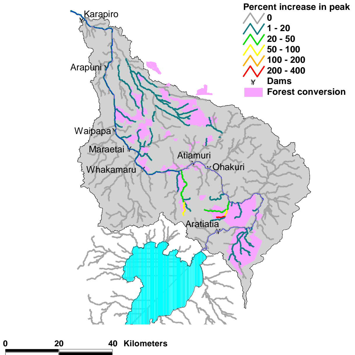
Figure 54 Percentage increase in peak flow for 100-year test rainfall event using the 1958 temporal pattern
