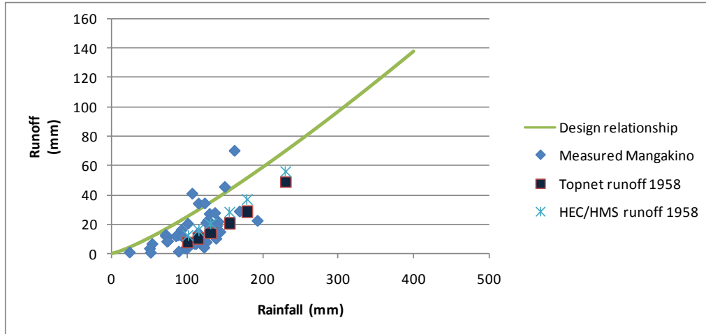
Figure 47 Measured storm runoff produced by total storm rainfalls and maximum design relationship in the Mangakino Stream compared to storm runoff into Maraetai reservoir predicted by HEC-HMS and TopNet models for rainfalls of 5 to 500 year ARI with 1958 temporal pattern
