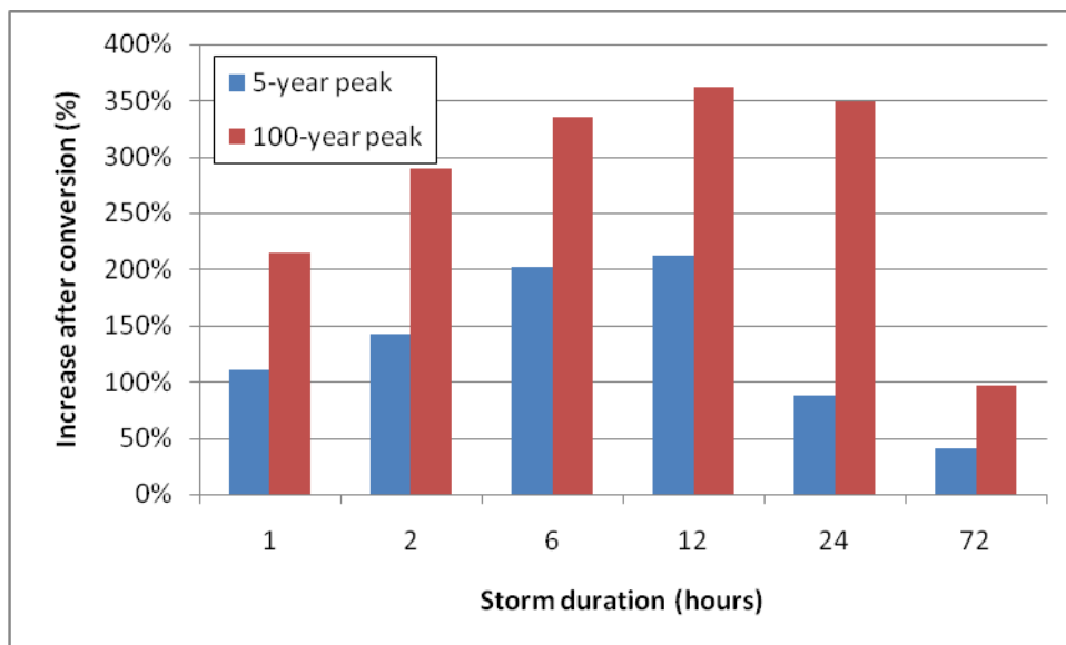
Figure 56 Pokaiwhenua at SH1: Increase in runoff peak after conversion based on HEC-HMS
