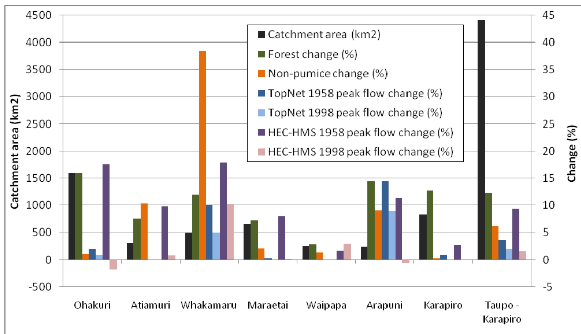
Figure 70 Landscape determinants of, and flooding response to, land cover change based on 100-year ARI storms modelled by TopNet and HEC-HMS. Depicted are: catchment area (black); percent of catchment area converted from forest to pasture (green); percent of converted forest underlain by non-pumice soils (orange); percent change in peak flood flow for 1958 (dark blue); and percent change in peak flood flow for 1998 (light blue). Post-conversion flood peaks are higher where more forest is converted, and where pumice is less extensive, all other factors being equal.
