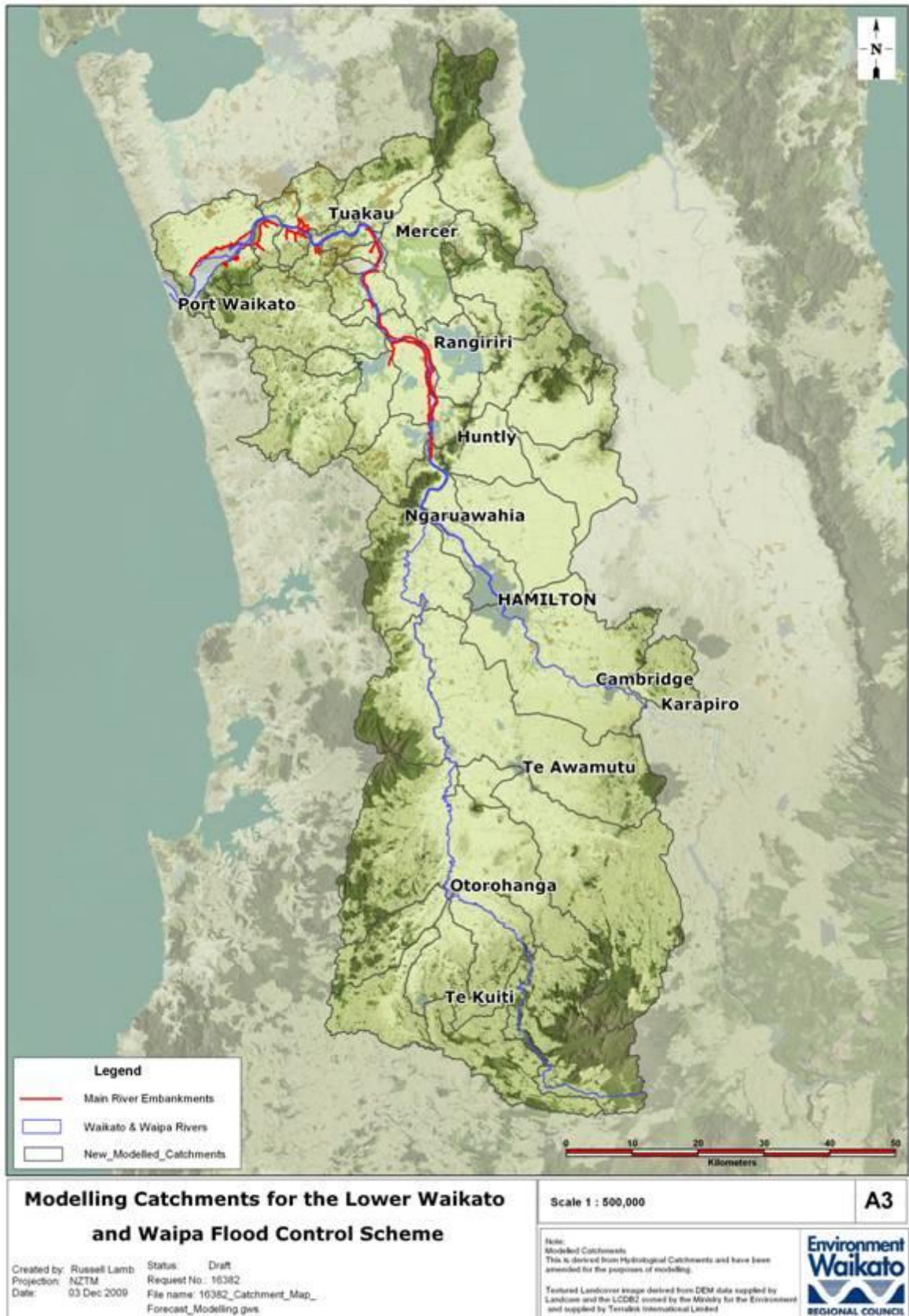
Figure 11 Location of the lower Waikato flooding simulations
