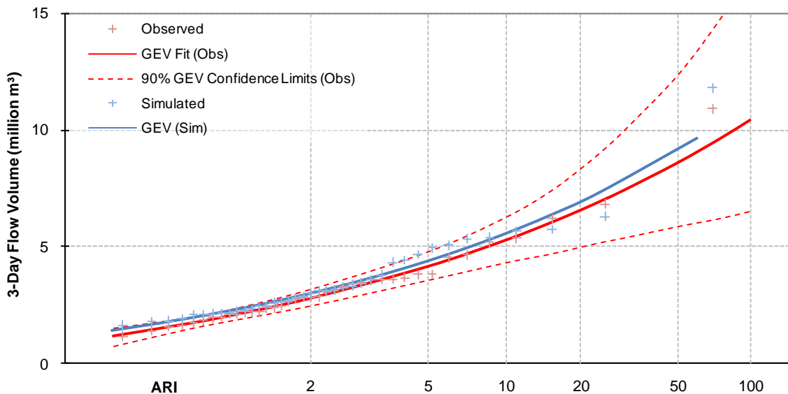
Figure 23 Distribution of observed and simulated 3-day flow volume annual maxima for Waio tapu at Reporoa calibration (using Gringorton plotting positions)
