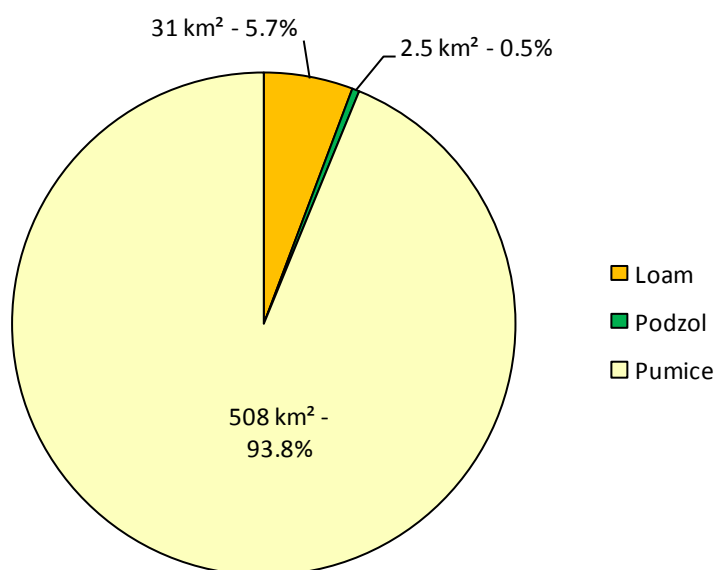
Figure 4 Soil type distribution of land identified for potential deforestation
