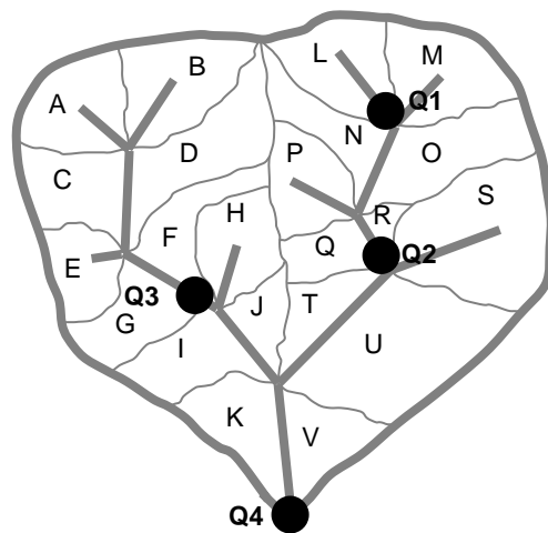
Figure 7 Schematic of TopNet model Each letter indicates a sub-basin, and the symbols Q1 – Q4 indicate the location of flow recording sites.
