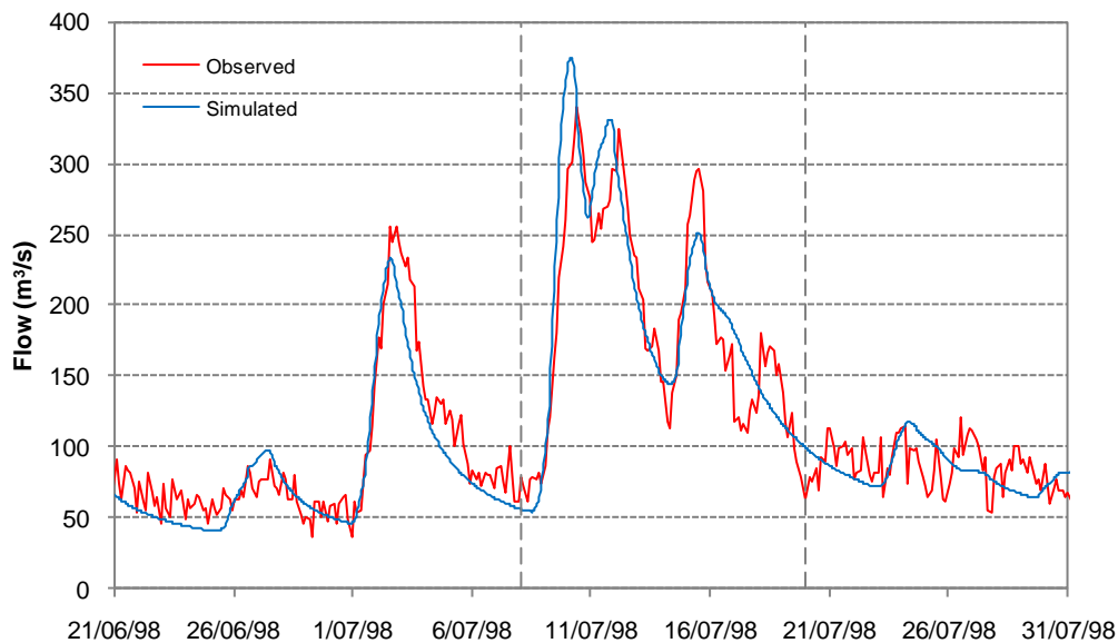
Figure 43 Simulated and observed inflow to the catchment between Lakes Whakamaru and Karapiro for the July 1998 flood event (24-hour moving mean)
