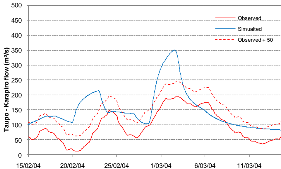
Figure 41 Observed difference between Taupo and Karapiro outflows and simulated catchment flow for the February 2004 flood event (72-hour moving means)
