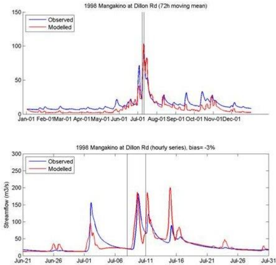
Figure 19 TopNet validation plot for 1998 flood, Mangakino at Dillon Road. Top panel shows observed and modelled 72-h moving mean flows in m^3 s^{-1} ; Bottom panel shows observed and modelled hourly flows in m^3 s^{-1}
