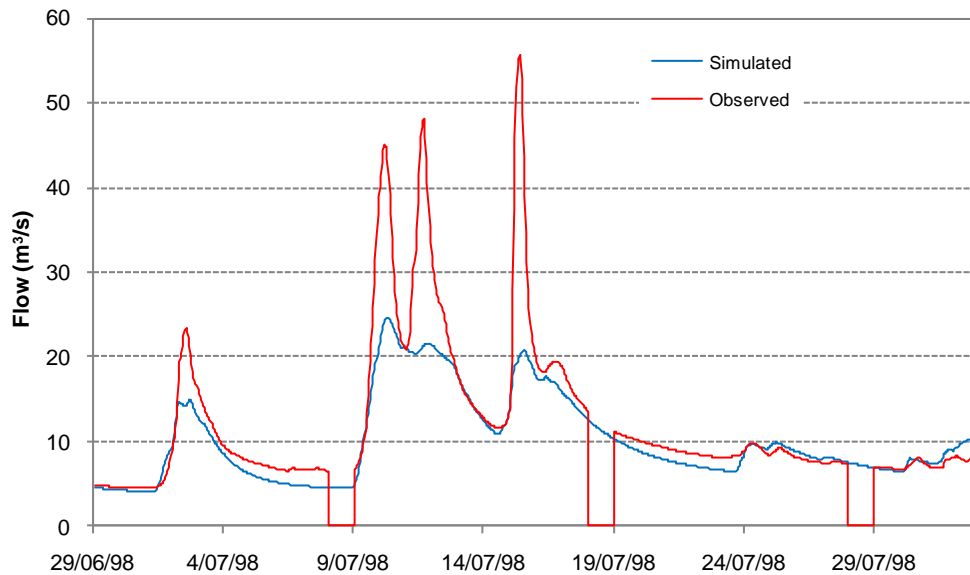
Figure 29 Observed and simulated flow at Tahunaatara at Ohakuri calibration for the July 1998 flood
