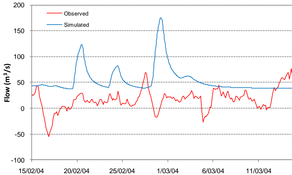
Figure 42 Simulated and “observed” inflow to the catchment between Lakes Taupo and Whakamaru for the February 2004 flood event (24-hour moving mean)
