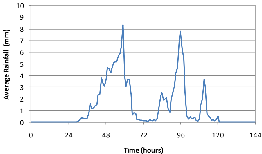
Figure 52 Average catchment rainfall (Starting at 09:00 on 7 July 1998)
