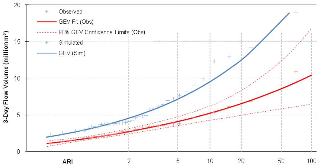
Figure 13 Distribution of observed and simulated 3-day flow volume annual maxima for Waiotapu at Reporoa calibration (using Gringorton plotting positions)
