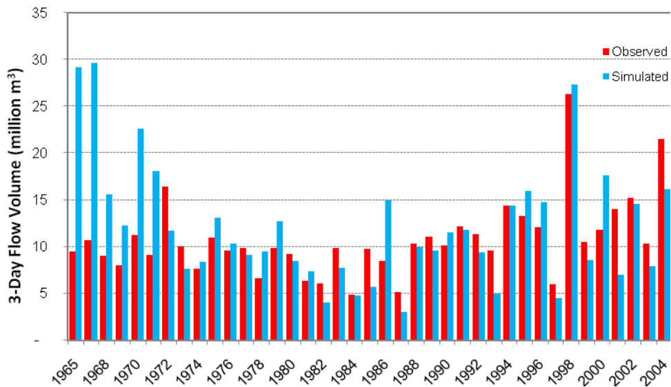
Figure 14 Observed and simulated 3-day flow volume annual maxima for Mangakino at Dillon Road calibration
