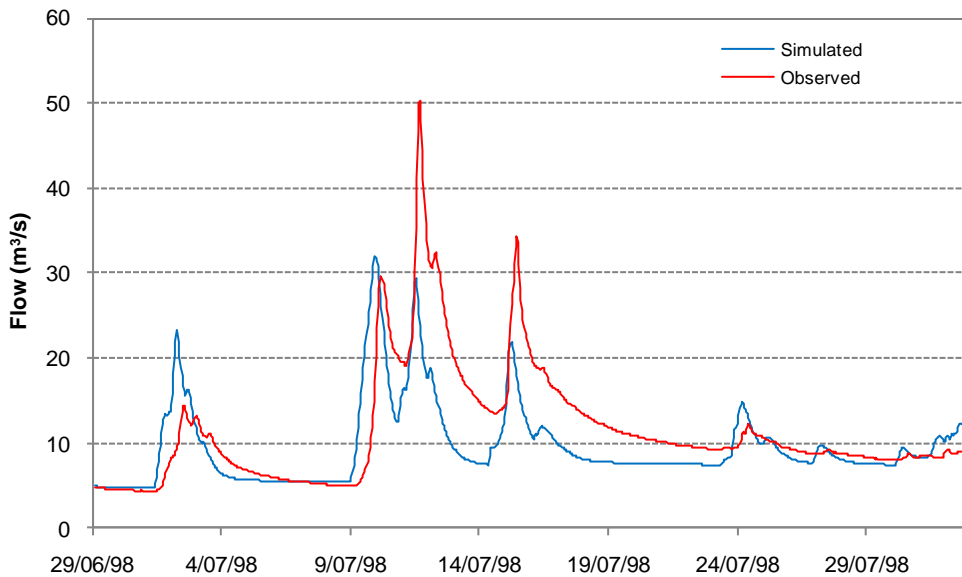
Figure 37 Observed and simulated flow at Pokaiwhenua at Puketuru calibration for the July 1998 flood
