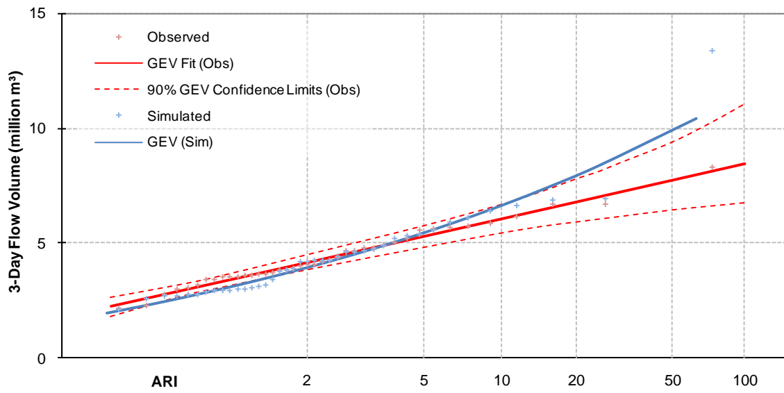
Figure 27 Distribution of observed and simulated 3-day flow volume annual maxima for Tahunaatara at Ohakuri calibration (using Gringorton plotting positions)
