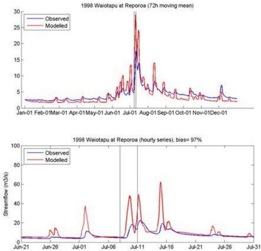
Figure 17 TopNet validation plot for 1998 flood, Waiotapu at Reporoa. Top panel shows observed and modelled 72-h moving mean flows in m^3s^{-1} ; Bottom panel shows observed and modelled hourly flows in m^3s^{-1}
