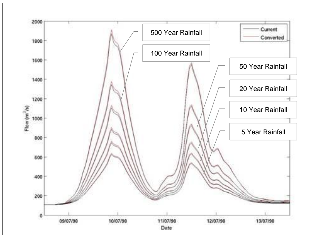
Figure 64 Simulated Taupo-Karapiro inflow hydrographs for the 6 synthetic rainfall events under current (black) and converted (red) land use scenarios, TopNet, 1998 events
