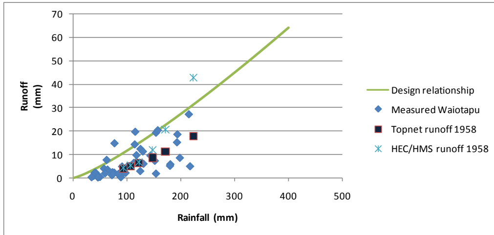
Figure 45 Measured storm runoff produced by total storm rainfalls and maximum design relationship in the Waiotapu Stream compared to storm runoff into Ohakuri reservoir predicted by HEC-HMS and TopNet models for rainfalls of 5 to 500 year ARI with 1958 temporal pattern
