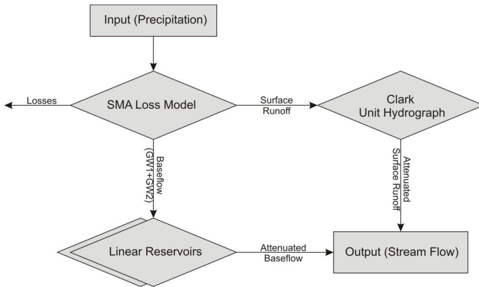
Figure 9 Interaction of HEC-HMS model components
