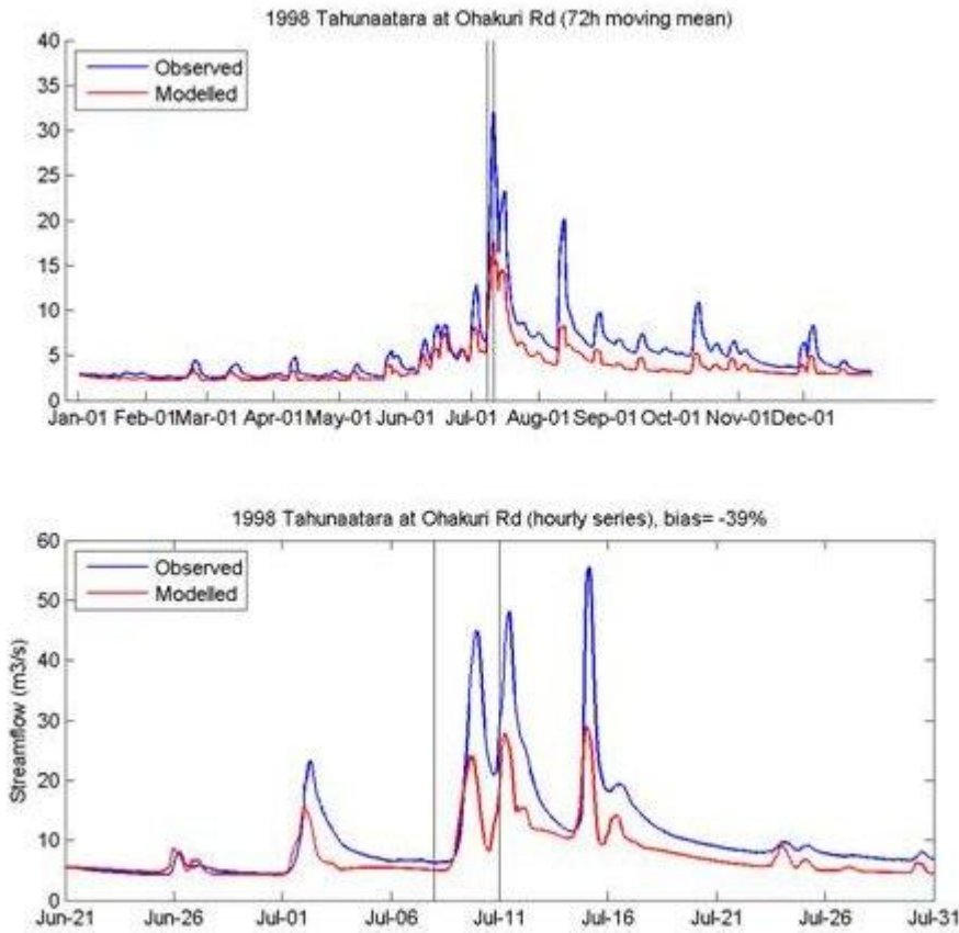
Figure 18 TopNet validation plot for 1998 flood, Tahunaatara at Ohakuri Road. Top panel shows observed and modelled 72-h moving mean flows in m^3s^{-1} ; Bottom panel shows observed and modelled hourly flows in m^3s^{-1}
