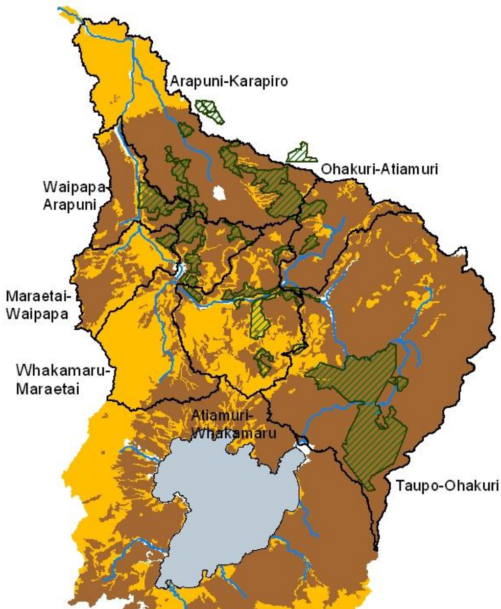
Figure 71 Regional map of general soil type, dam sub-catchment and areas of potential conversion. Dark brown is pumice soils; orange is non-pumice soils. Green striped regions indicate forest areas potentially subject to conversion to pasture.
