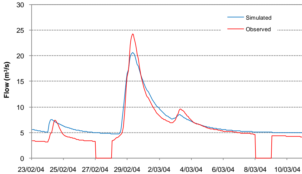
Figure 30 Observed and simulated flow at Tahunaatara at Ohakuri calibration for the February 2004 flood
