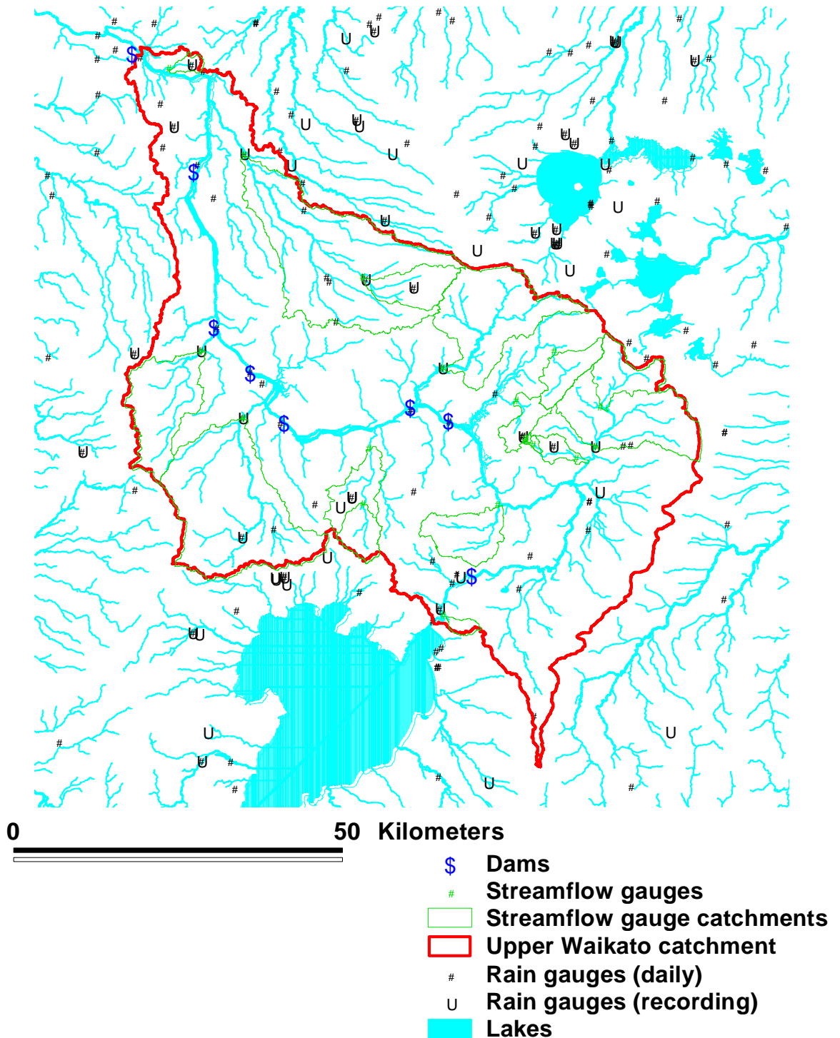
Figure 5 Streamflow and rainfall gauge locations
