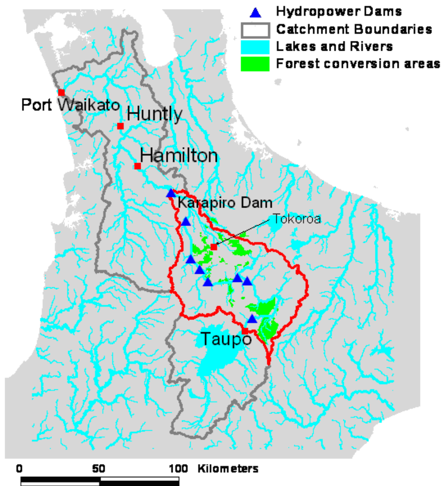
Figure 1 Overview of Waikato catchment, with the upper Waikato outlined in red, and the land use change areas shown in green
