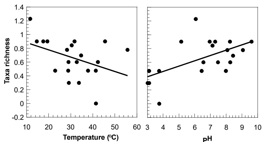
Figure 6. Log (x+1) taxa richness from 20 stream sites with various levels of geothermal influence in the Taupo Volcanic Zone against temperature and pH.
