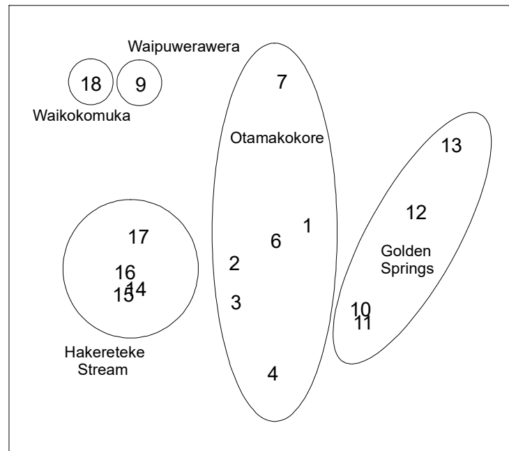
Figure 7. Ordination diagram based on MDS of macrofaunal composition from 16 stream sites with various levels of geothermal influence in the Taupo Volcanic Zone. Numbers correspond to site numbers (see Figures 1-4). Stress = 0.06.
