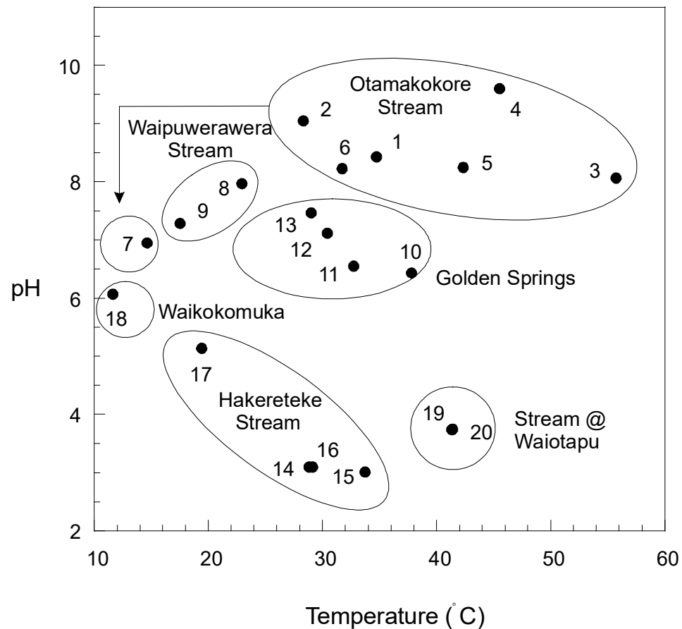
Figure 5. Temperature and pH recorded from 20 stream sites with various levels of geothermal influence in the Taupo Volcanic Zone (see Figures 1-4 for site numbers).
