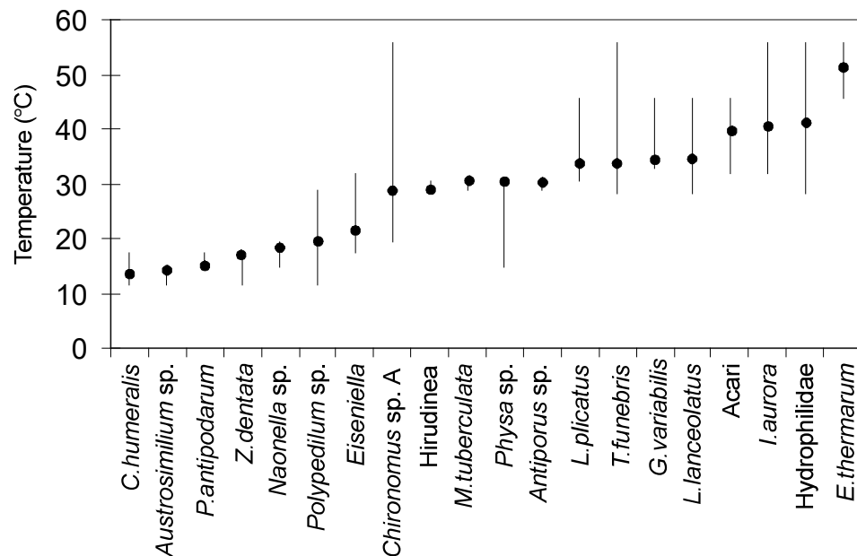
Figure 9. Weighted average optima (dots) and maximum and minimum (bars) temperatures recorded for dominant species.
