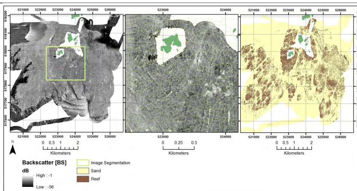
Figure 3-12 An example of image segmentation of multibeam backscatter. A) Multibeam backscatter image B) Image segmentation shown by green outlines C) Image classification of segments based on object textural and spatial parameters (slope, rugosity etc).
