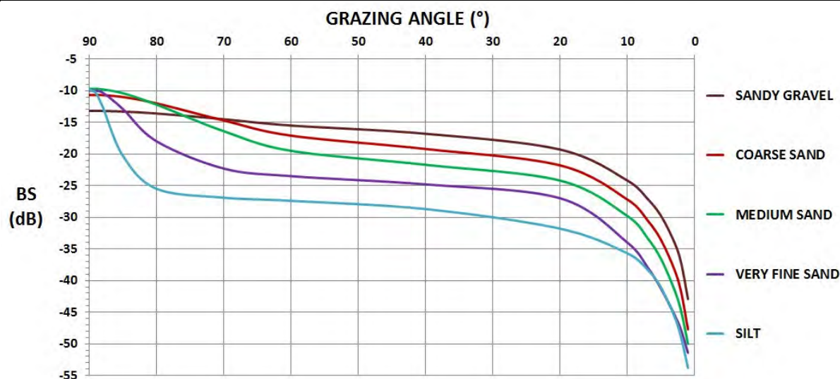
Figure 3-6 Backscatter Strength (BS) versus grazing angle for different classes of sediment at 100 kHz. Data from: University of Washington Applied Physics Laboratory, high-frequency ocean environmental acoustic models, APL-UW TR 9407-AEAS 9501, October 1994.
