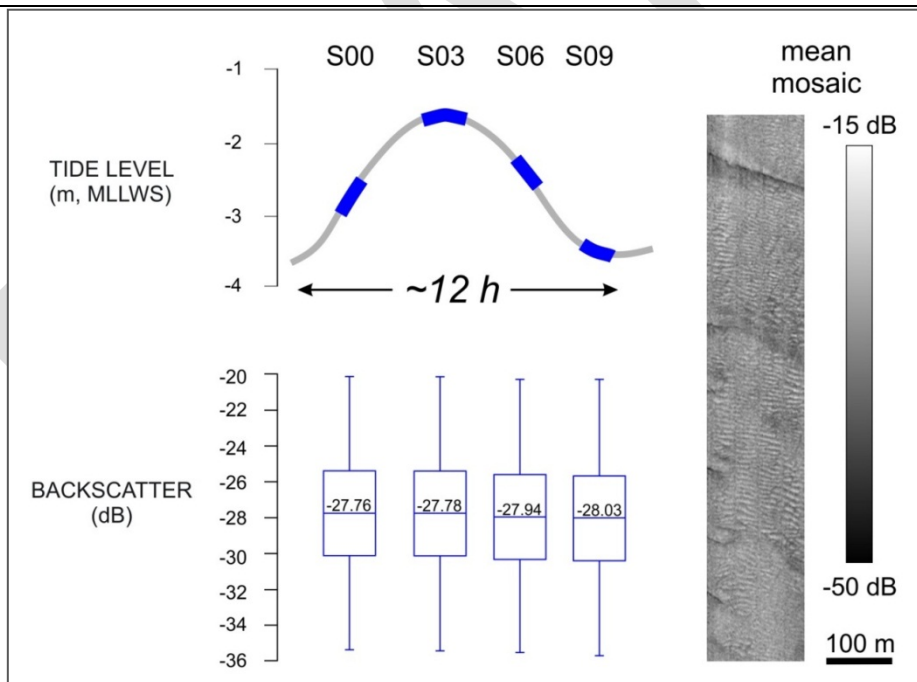
Figure 3-5 Evaluation of Backscatter Strength (BS) variance from successive measurements during a tide cycle ( \sim 12h); 4 surveys of the same area with constant input and runtime parameters; boxplots of the BS data with mean values; for the four data sets, the statistics are calculated from each mosaics values (resolution = 1x1m) on the common rectangular area presented in the figure; very low dispersion of the 4 mean values: standard deviation = 0.1 dB; data from Kongsberg EM1002 MBES on RV Belgica.
